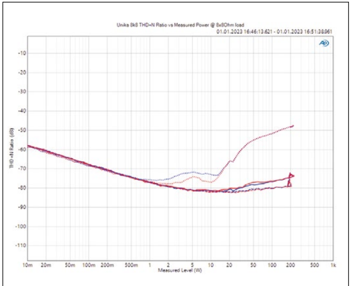
Distortions (THD+N) as a function of the output power (x-axis in W) at a load of 8 \times 8 \Omega . Measurements at 100 Hz (---), 1 kHz (—) and 6.3 kHz (···). Measurement for channels 1 and 2 (Fig. 11)
