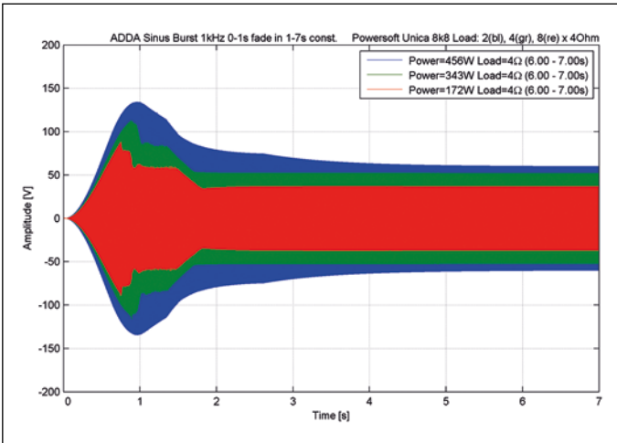
Burst measurement with a sine signal of 1 kHz for a one-, two-, four- or eight-channel load of 4 Ω. The measured curve is identical for a one- or two-channel load (Fig. 18)
