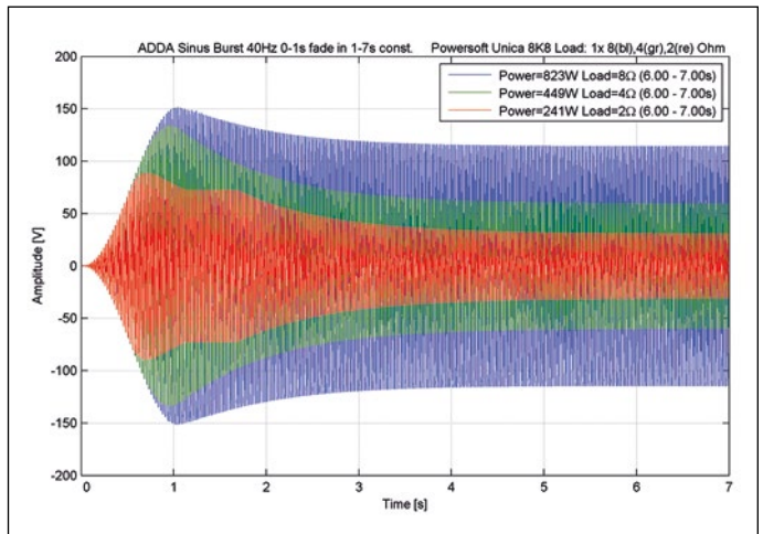
Burst measurement with a single-channel 40 Hz sine signal for loads of 2 Ω, 4 Ω or 8 Ω (Fig. 17)
