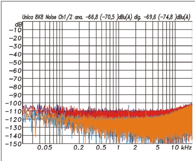
Noise level at the output measured exemplarily for channels 1 and 2. When using the analogue inputs, the noise level is -66.8 dBu and 70.5 dBu(A). With a digital input, the results are 69.6 dBu and -74.8 dBu. The maximum signal level is 43.3 dBu (Fig. 7)
