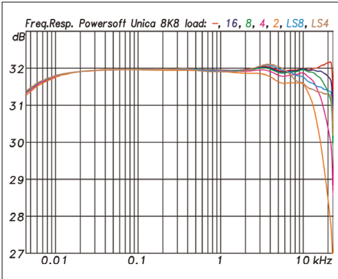
Frequency responses measured with loads of 2, 4, 8 and 16 Ω, without load and with typical loudspeaker impedances for 4 Ω and 8 Ω nominal impedance (Fig. 5)
