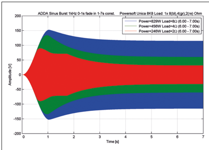
Burst measurement with a single-channel 1 kHz sine signal for loads of 2 Ω, 4 Ω or 8 Ω. The burst signal is faded in within the first second, which prevents overshooting of the limiter (Fig. 16)
