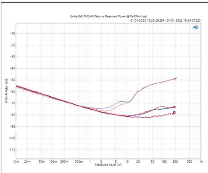
Distortions (THD+N) as a function of the output power (x-axis in W) at a load of 8 \times 4 \Omega . Measurements at 100 Hz (---), 1 kHz (—) and 6.3 kHz (···). Measurement for channels 1 and 2 (Fig. 12)
