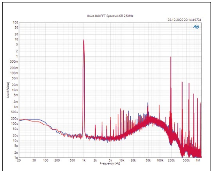
FFT spectrum for the output signal measured with 2.5 MHz sample rate. At 1 kHz, the useful signal with a voltage of 10 V can be identified. Remnants of the PWM switching frequency in the order of 1 V are found at 192 kHz and its integer multiples (Fig. 9)
