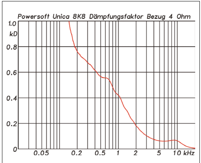
Damping factor related to 4 Ω measured exemplarily for channel 1 (Fig. 8)
