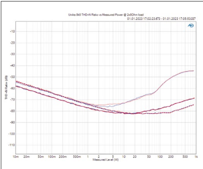
Distortions (THD+N) as a function of the output power (x-axis in W) at a load of 2 \times 8 \Omega . Measurements at 100 Hz (---), 1 kHz (—) and 6.3 kHz (···). The distortion values increase significantly from 6.3 kHz onwards (Fig. 10)
