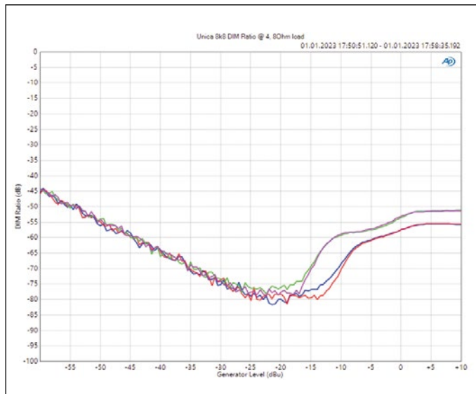
Transient intermodulation distortions (DIM100) as a function of the input level measured exemplarily for channels 1 and 2 with a load of 4 Ω (blue, red) and of 4 × 8 Ω (green, magenta) (Fig. 15)
