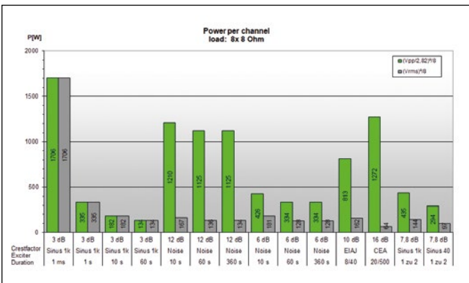
Power for different signal types Unica 8k8 with 8 Ω per channel with simultaneous load of all channels (Fig. 20)
