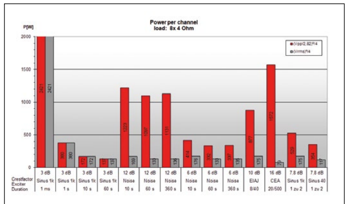
Power for different signal types Unica 8k8 with 4 Ω per channel with simultaneous load of all channels (Fig. 21)
