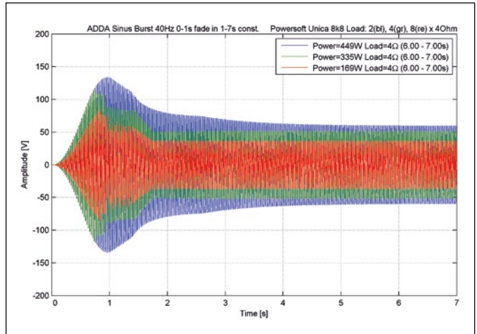
Burst measurement with a sine signal of 40 Hz for a one-, two-, four- or eight-channel load of 4 Ω. The measured curve is identical for a one- or two-channel load (Fig. 19)
