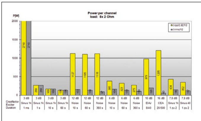
Power for different signal types Unica 8k8 with 2 Ω per channel with simultaneous load of all channels (Fig. 22)
