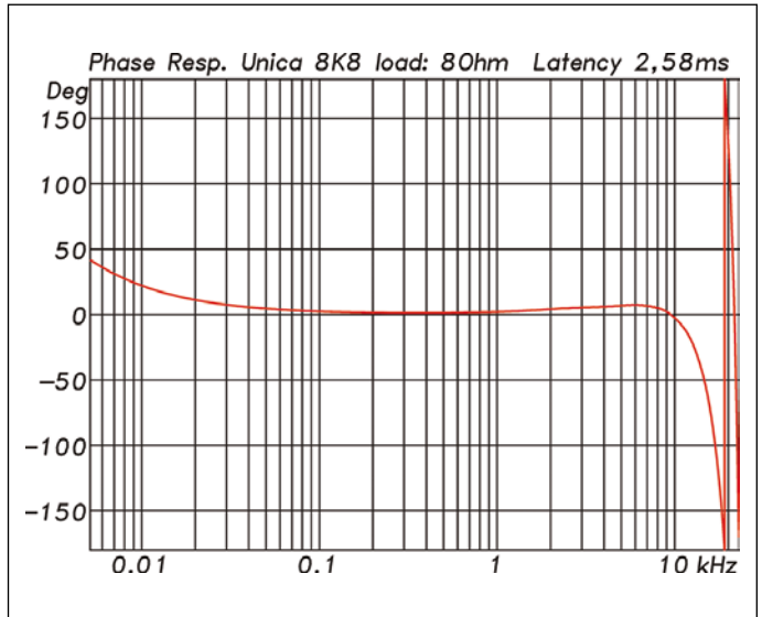
Phase response measured with a load of 8-Ω. The base latency is 2.58 ms (Fig. 6)
