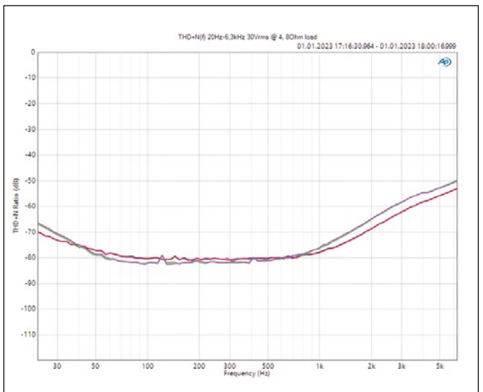
Distortions (THD+N) depending on the frequency exemplary for channels 1 and 2 at an output voltage of 30 V_{rms} with a load of 4 \Omega (red, blue) and of 8 \Omega (green, purple) (Fig. 13)
