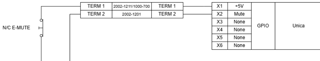
Figure 33 – Unica Normally Closed E-Mute Application Example
