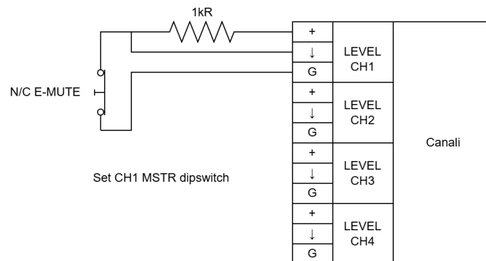
Figure 21 – Canali Normally Closed E-Mute Circuit using VCA
