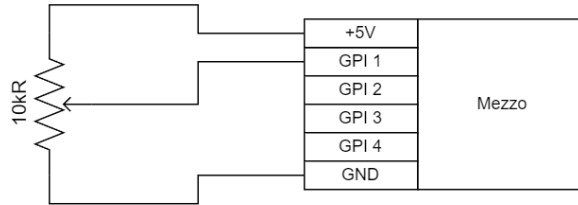
Figure 5 – Mezzo VCA Circuit
