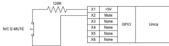
Figure 32 – Unica Normally Closed E-Mute Circuit
