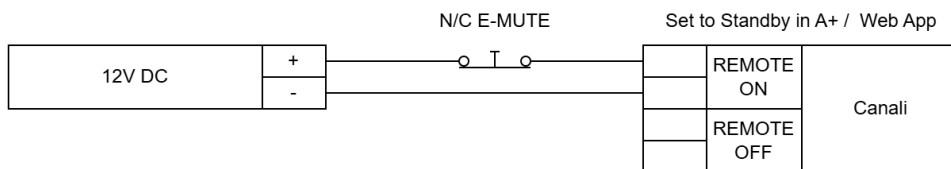
Figure 17 – Canali Normally Closed E-Mute Circuit using Remote ON
