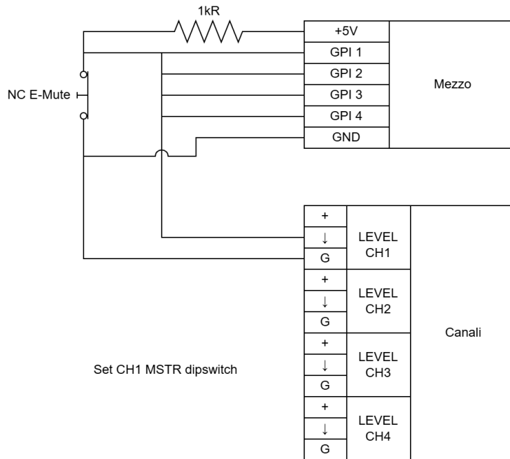
Figure 44 – Mezzo & Canali Normally Closed E-Mute Circuit
