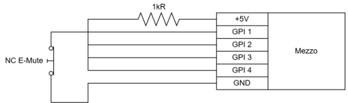
Figure 11 – Mezzo Normally Closed E-Mute Circuit
