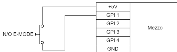
Figure 37 – DMD Normally Open Emergency Mode Trigger Circuit
