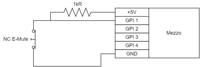
Figure 38 – DMD Normally Closed Emergency Mode Trigger Circuit
