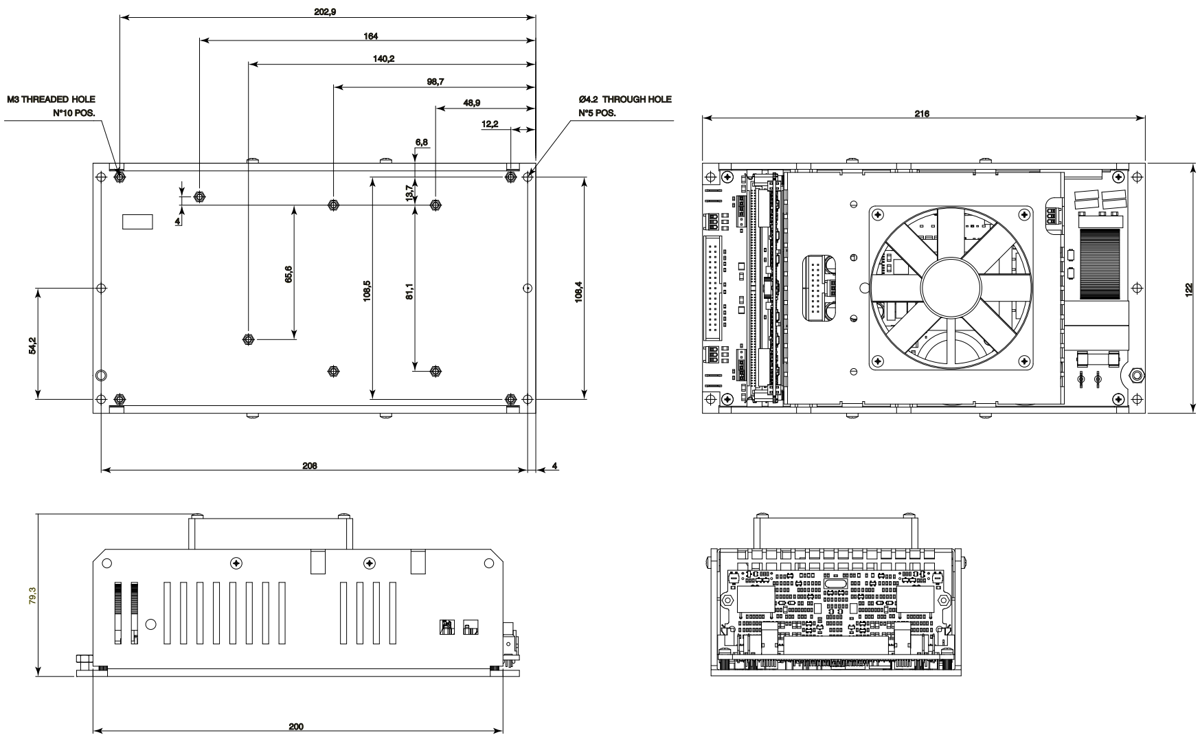
FIGURE 2: DigiMod 2004PFC2 mechanical drawings. All dimensions in millimeters.
